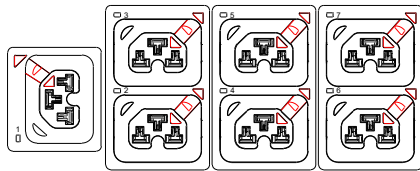
Locking C39 sockets
